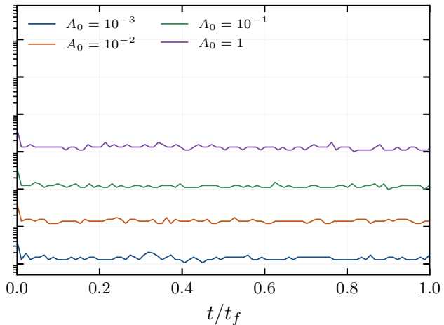
(b) Field-loop sequence
