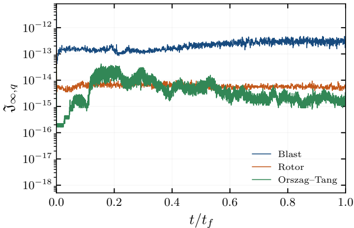
(a) Shock-dominated flows
